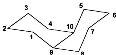
Figure 1. Numbering used for cis -decalin.
