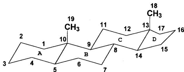
Figure 2. Numbering used for 5 \alpha -androstane.
